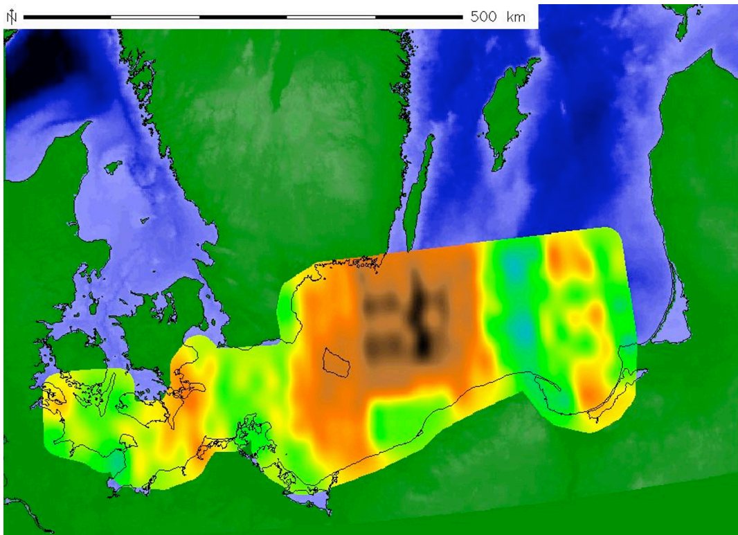
Figure 2. Wind speed raster grid map (shaded zone extending eastward from southeastern Jutland) interpolated from 10' data points in GRASS 5.7. Lighter is lower velocity and darker is higher velocity.
