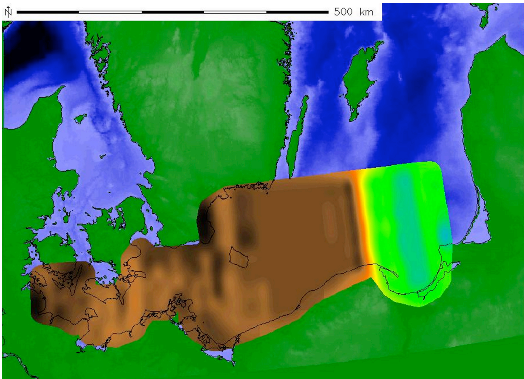
Figure 3. Wind direction raster grid map, interpolated from 10' data points in GRASS 5.7. Lightest is an east wind, darkest is a west wind, and light brown-yellow (medium gray) is a southwest wind.
